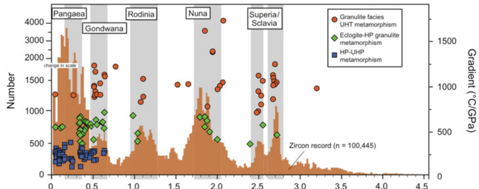
FIGURE 1 Histogram of U–Pb crystallization ages for over 100,000 detrital zircon grains (Voice et al. 2011) and metamorphic thermal gradients (Brown
