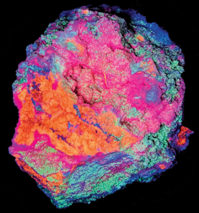
Rock specimen (15 cm across) from Mt. St. Hilaire, Quebec, Canada. Under ultraviolet illumination, sodalite emits orange, albite pink-red, presumable gaidonnayite green, and pectolite blue-purple. IMAGES BY GLENN WAYCHUNAS.
